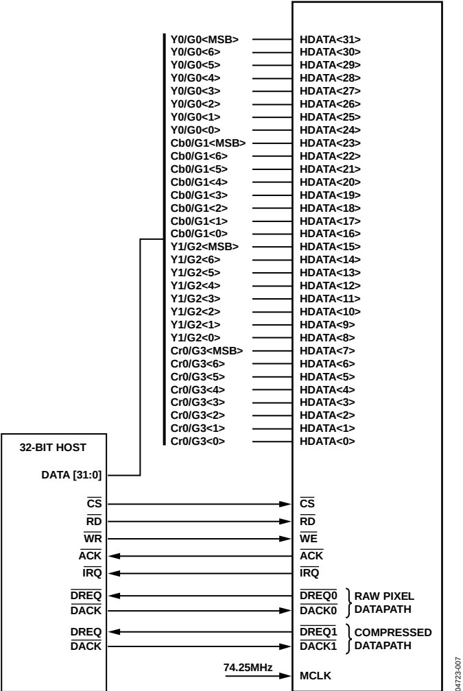
Figure 29. Host Interface—Pixel Interface Mode
