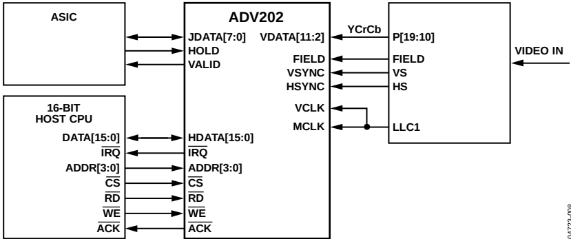
Figure 30. JDATA Application
