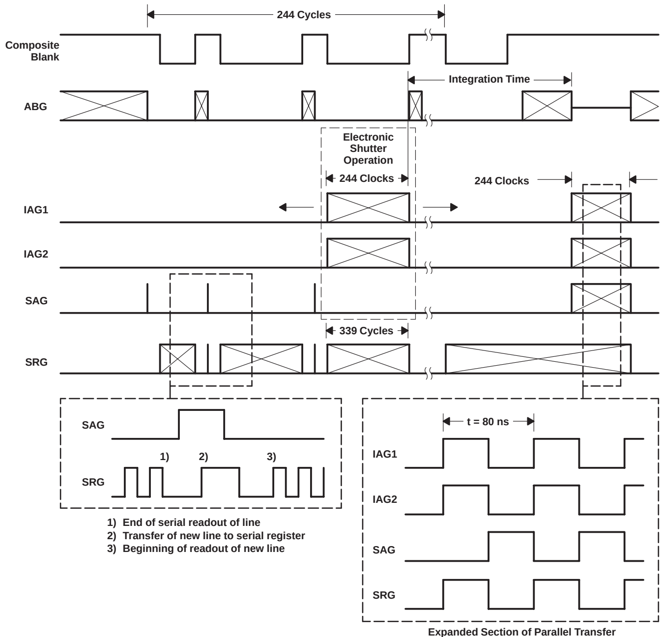
Figure 3. Timing Diagram
