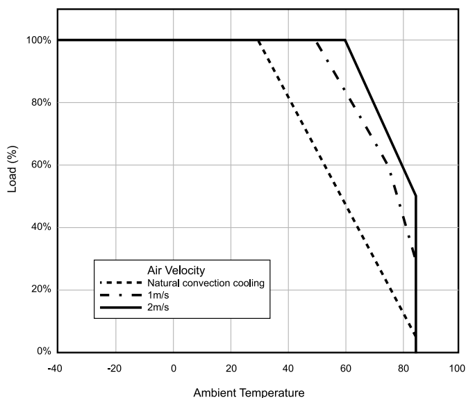
PAQ100 Derating Curve
