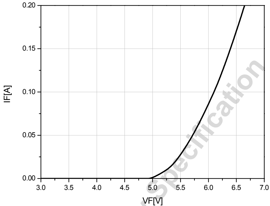
Fig 3-1. Forward Voltage vs. Forward Current , Ta=25°C (@LED)
