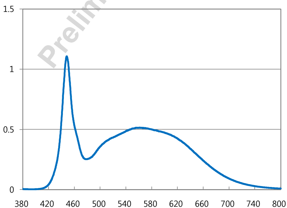
Fig 1-2. Relative Spectral Distribution vs. Wavelength Characteristic – 4700K, 7000K
