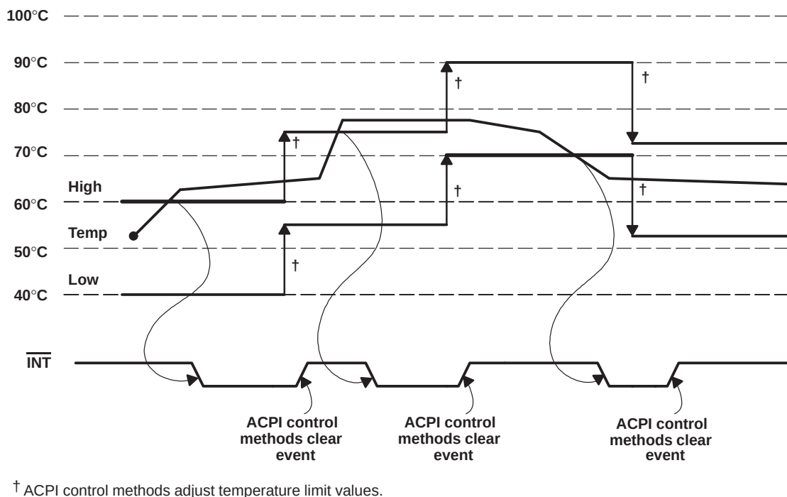
Figure 15. Examples of Temperature Interrupt Events
