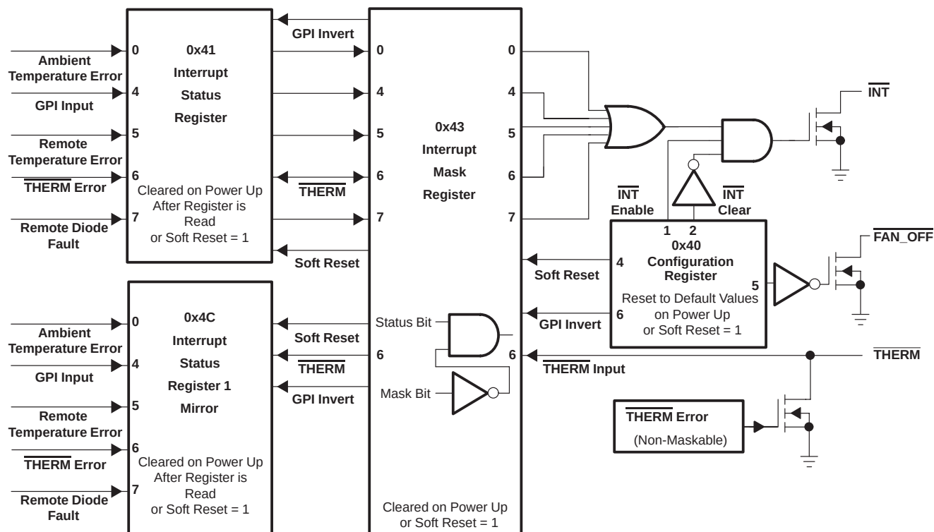
Figure 22. Interrupt Structure
