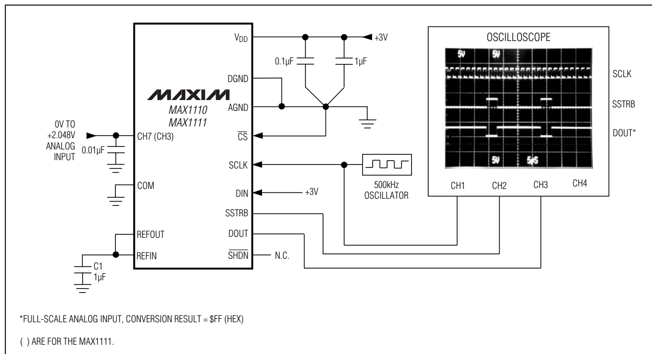
Figure 5. Quick-Look Circuit
