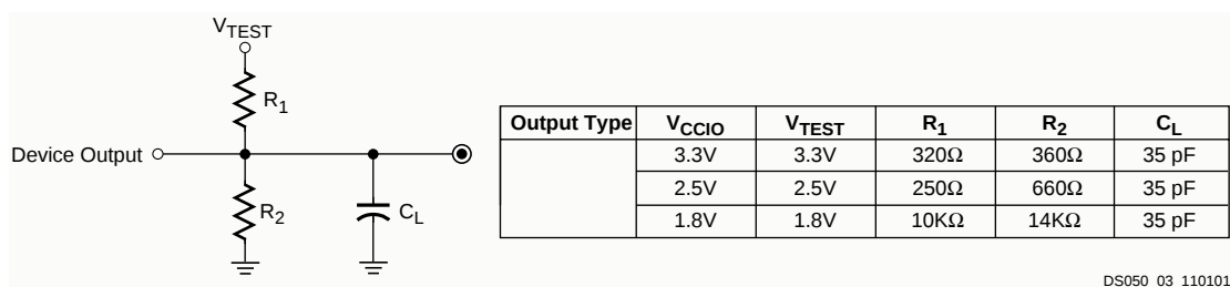
Figure 3: AC Load Circuit
