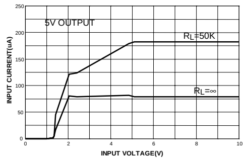
Figure 3. Input Current
