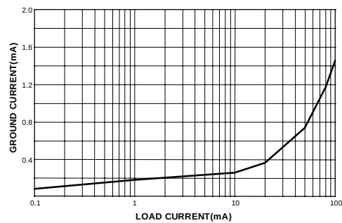
Figure 1. Quiescent Current
