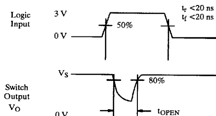
Figure 4. Break-Before-Make Interval
