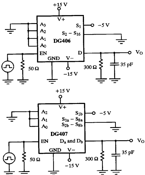
Figure 3. Enable Switching Time
