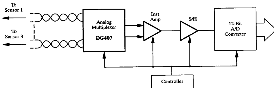
Figure 6. Measuring low-level analog signals is more accurate when using a differential multiplexing technique.
