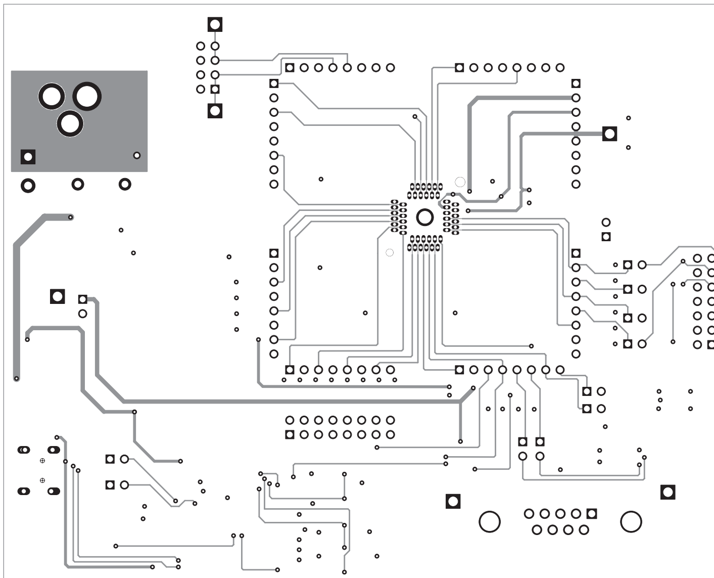
Figure 5. Layer-2 Routing
