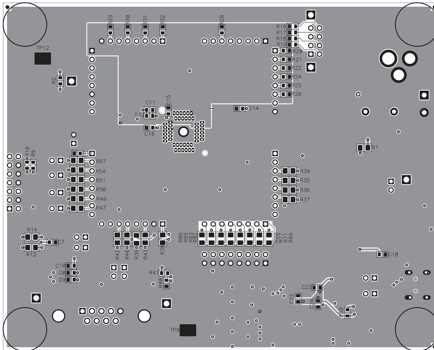
Figure 7. Bottom-Side Placement/Routing
