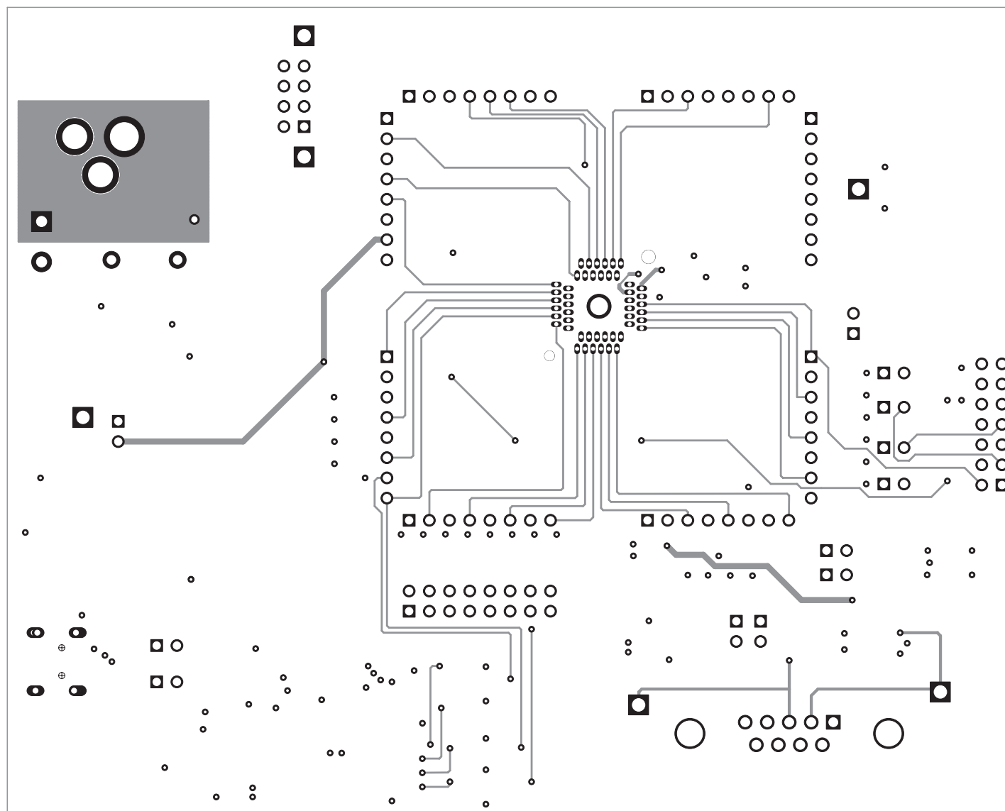
Figure 6. Layer-3 Routing
