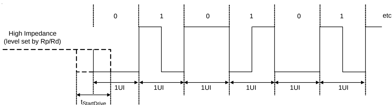
Figure 5. BMC Encoded Start of Preamble
