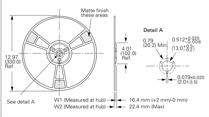
Figure 8. Reel Dimensions in Inches (mm)
