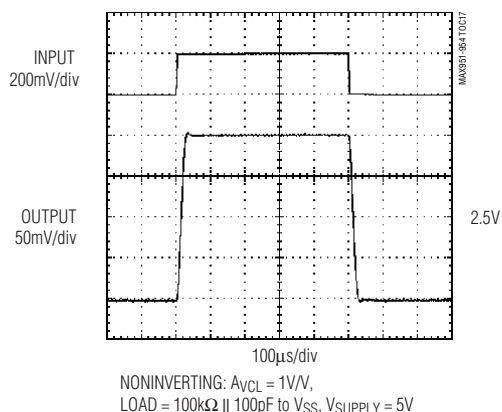
MAX952/MAX954 OP AMP SMALL-SIGNAL TRANSIENT RESPONSE
