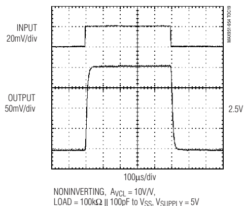
MAX952/MAX954 OP AMP SMALL-SIGNAL TRANSIENT RESPONSE
