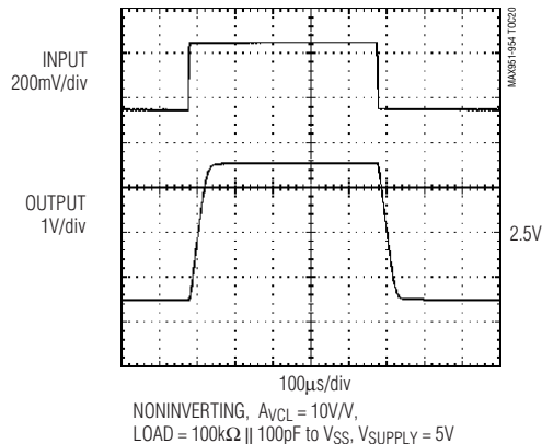
MAX952/MAX954 OP AMP LARGE-SIGNAL TRANSIENT RESPONSE
