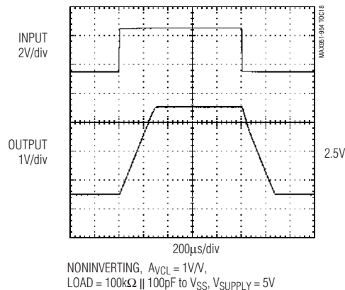
MAX952/MAX954 OP AMP LARGE-SIGNAL TRANSIENT RESPONSE
