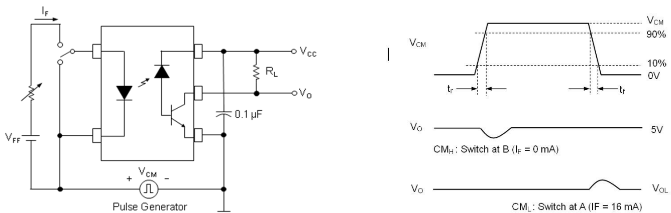
Figure 10 Transient Immunity Test Circuit & Waveform
