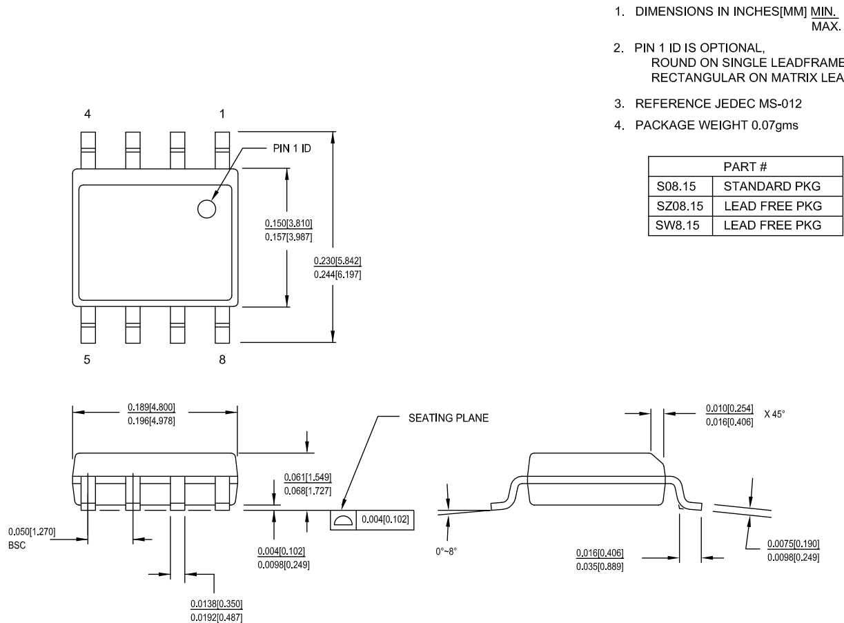
Figure 19. 8-pin SOIC (150 Mils) Package Outline, 51-85066
