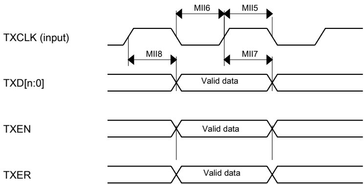
Figure 26. RMII/MII transmit signal timing diagram
