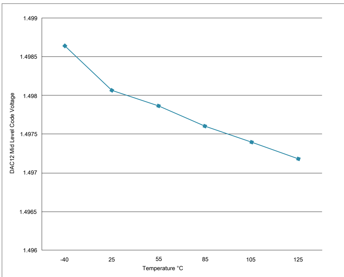
Figure 25. Offset at half scale vs. temperature
