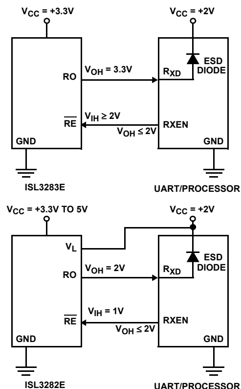
FIGURE 6. USING V_L PIN TO ADJUST LOGIC LEVELS
