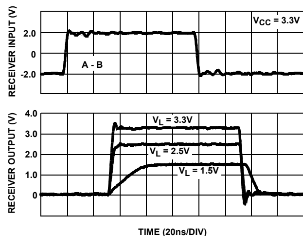
FIGURE 19. RECEIVER WAVEFORMS
