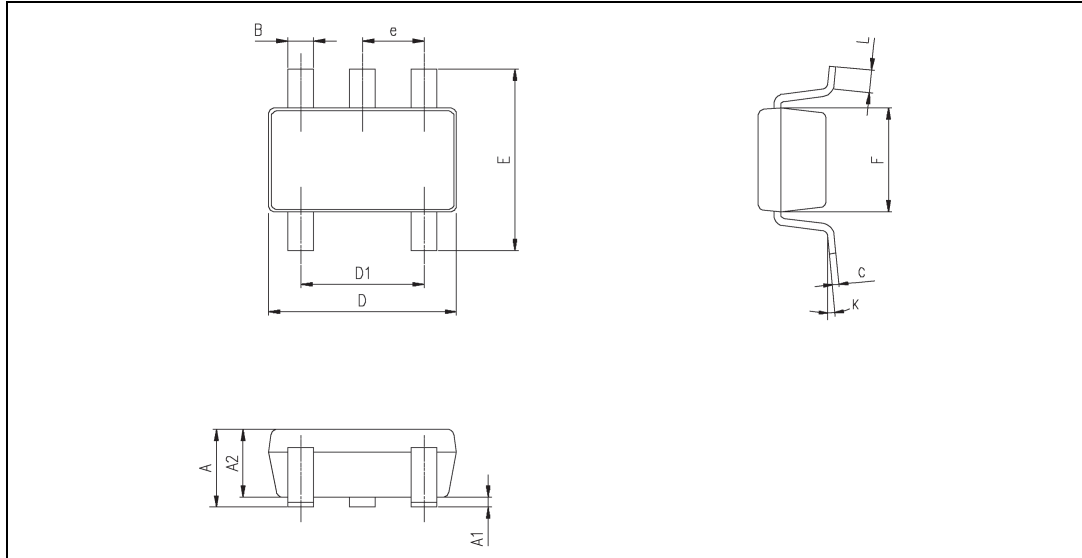
Figure 43. SOT23-5 package mechanical drawing
