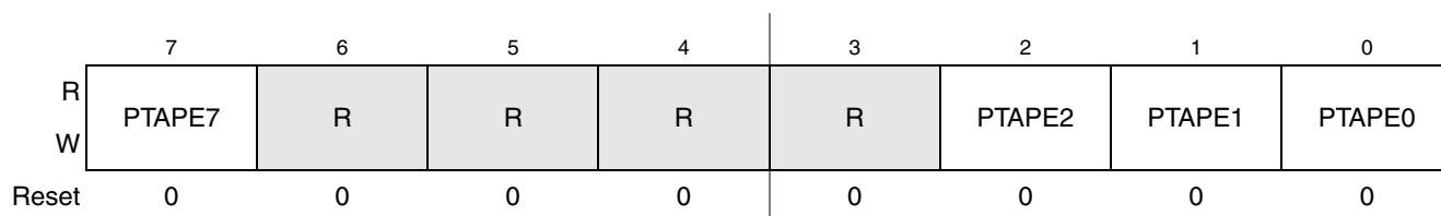
Figure 6-12. Internal Pullup Enable for Port A (PTAPE) 1
