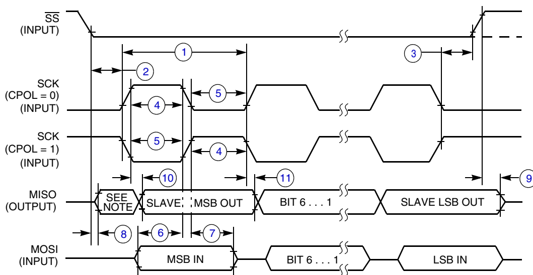
Figure A-17. SPI Slave Timing (CPHA = 0)
