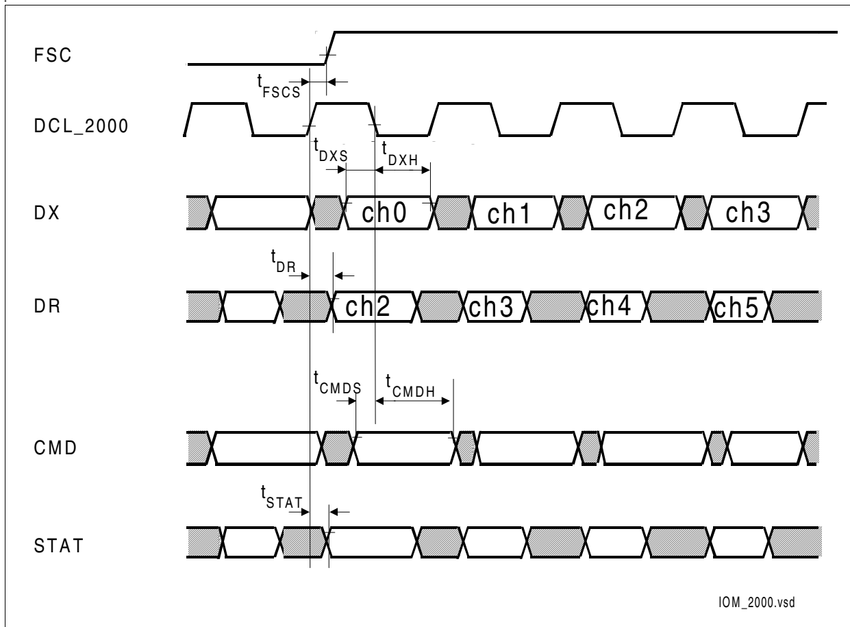
Figure 25 IOM-2000 Timing
