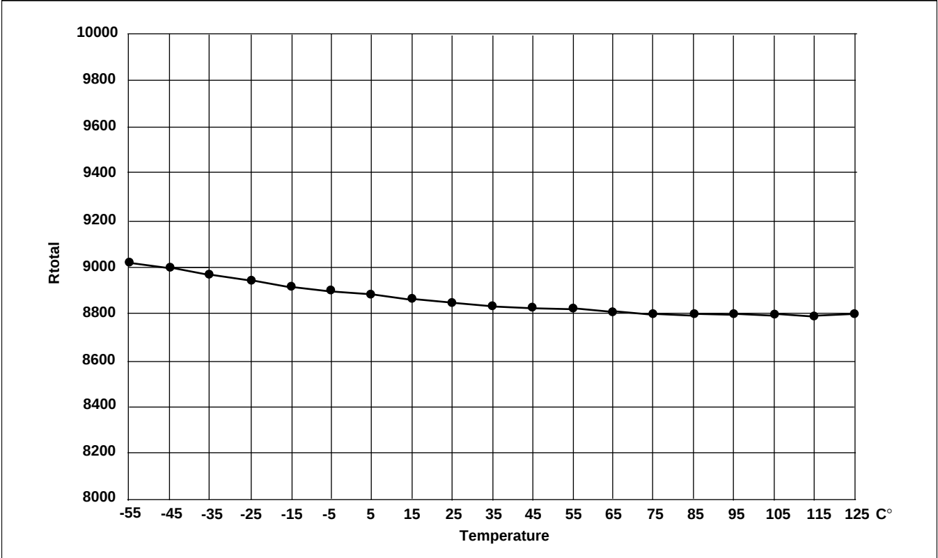
TYPICAL RTOTAL vs. TEMPERATURE
