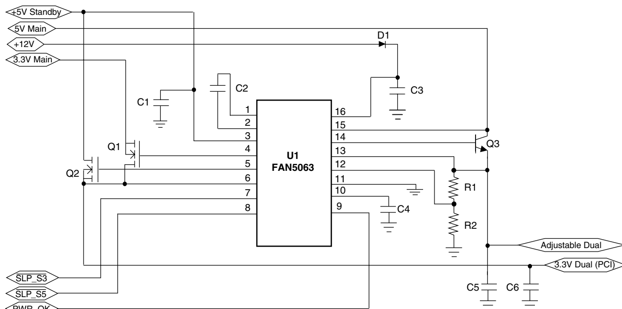
Figure 4. ACPI Selector
