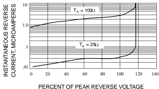
Fig. 3-TYPICAL REVERSE CHARACTERISTICS
