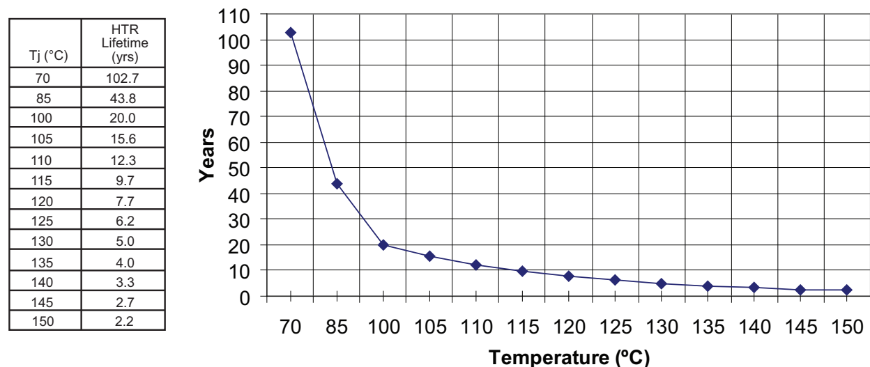
Figure 2-1 • High Temperature Data Retention (HTR) for FPGA/FlashROM
