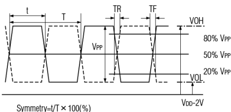
Figure 5) Output Waveform (1)
