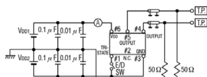
Figure 1) Test Circuit (1)
