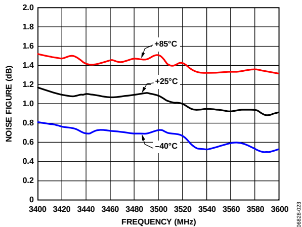
Figure 23. Noise Figure vs. Temperature
