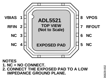
Figure 2. Pin Configuration
