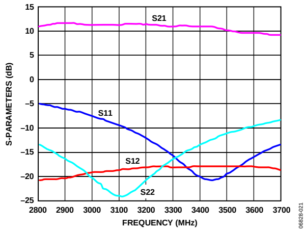
Figure 21. Typical S-Parameters, Log Magnitude
