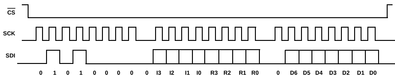
FIGURE 16. THREE BYTE WRITE SEQUENCE
