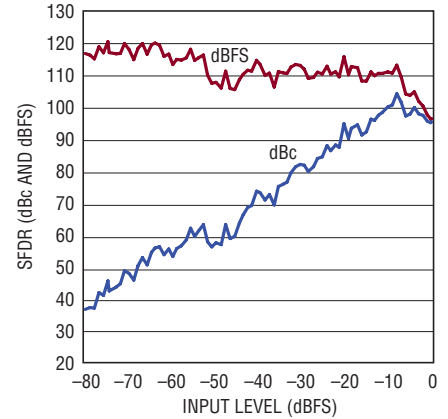
LTC2192: SFDR vs Input Level, f_{IN} = 70\text{MHz} , 65Mps, 2V Range
