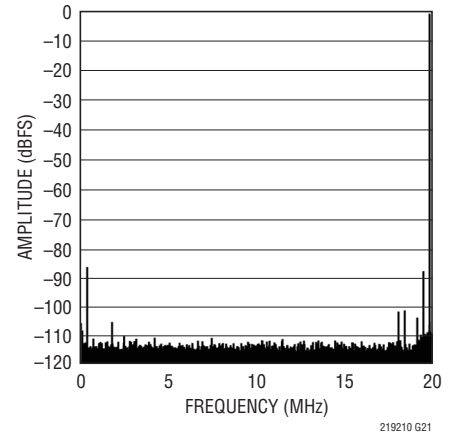
LTC2191: 64k Point FFT, f_{IN} = 140\text{MHz} , -1\text{dBFS} , 40\text{Mps}
