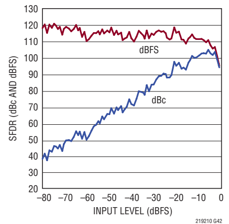
LTC2190: SFDR vs Input Level, f_{IN} = 70\text{MHz} , 25\text{Mpsps} , 2\text{V} Range
