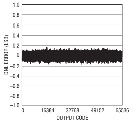
LTC2191: Differential Nonlinearity (DNL)
