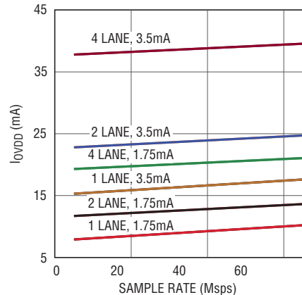
LTC2192: I_{VDD} vs Sample Rate, 5MHz, -1dBFS Sine Wave on Each Input
