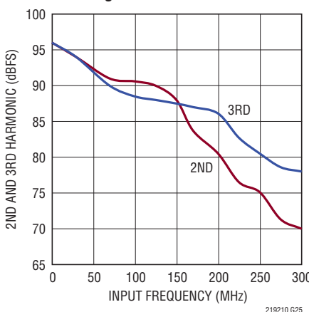
LTC2191: 2nd, 3rd Harmonic vs Input Frequency, -1\text{dBFS} , 40\text{Mps} , 2\text{V} Range
