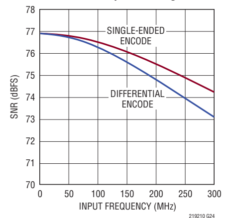
LTC2191: SNR vs Input Frequency, -1\text{dBFS} , 40\text{Mps} , 2\text{V} Range
