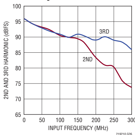
LTC2191: 2nd, 3rd Harmonic vs Input Frequency, -1\text{dBFS} , 40\text{Mps} , 1\text{V} Range
