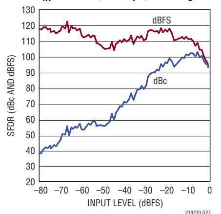
LTC2191: SFDR vs Input Level, f_{IN} = 70\text{MHz} , 40\text{Mps} , 2\text{V} Range
