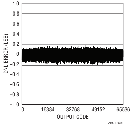
LTC2192: Differential Nonlinearity (DNL)
