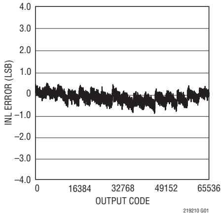
LTC2192: Integral Nonlinearity (INL)
