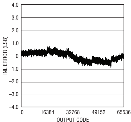
LTC2191: Integral Nonlinearity (INL)
