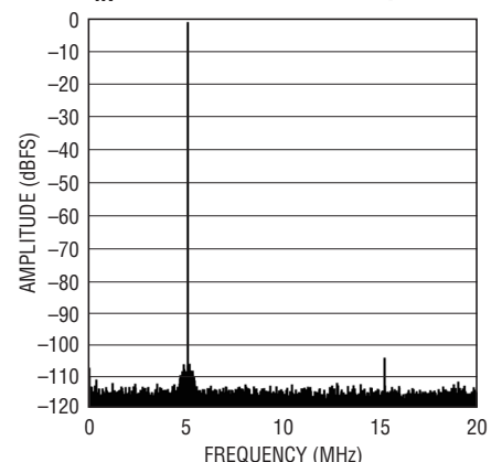
LTC2191: 64k Point FFT, f_{IN} = 5\text{MHz} , -1dBFS, 40Mps
