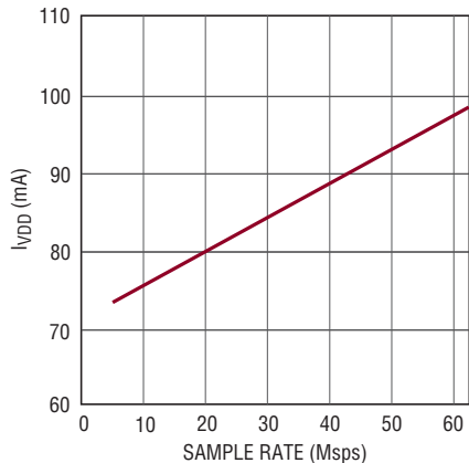
LTC2192: I_{VDD} vs Sample Rate, 5MHz, -1dBFS Sine Wave on Each Channel
