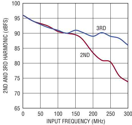
LTC2192: 2nd, 3rd Harmonic vs Input Frequency, -1dBFS, 65Mps, 1V Range
