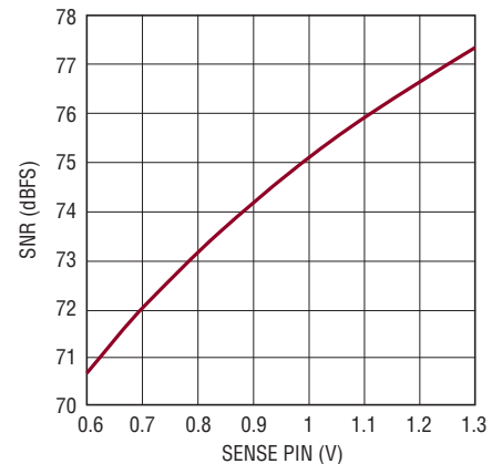
LTC2192: SNR vs SENSE, f_{IN} = 5\text{MHz} , -1dBFS
