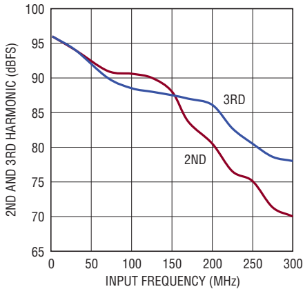
LTC2192: 2nd, 3rd Harmonic vs Input Frequency, -1dBFS, 65Mps, 2V Range
