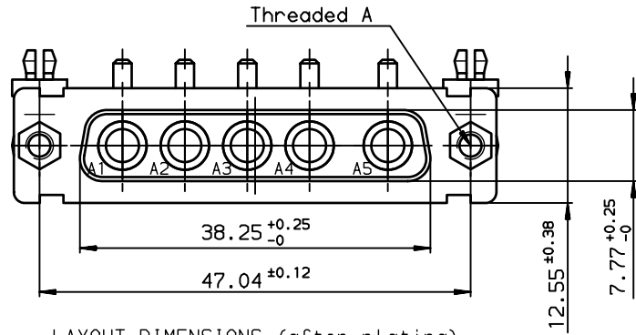
LAYOUT DIMENSIONS (after plating) CONNECTOR SIDE VIEW
