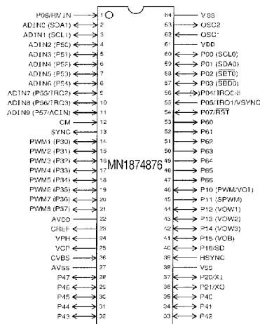
SDIP064-P-0750
