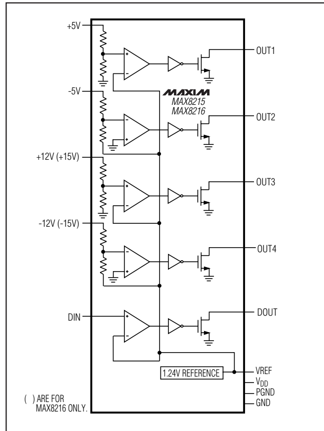
Figure 1. Block Diagram
