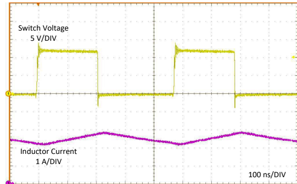
Figure 7-7. Typical PWM Switching Waveforms Without Spread Spectrum V_{IN} = 12V , V_{OUT} = 5V , I_{OUT} = 2.5A , f_{SW} = 2100kHz
