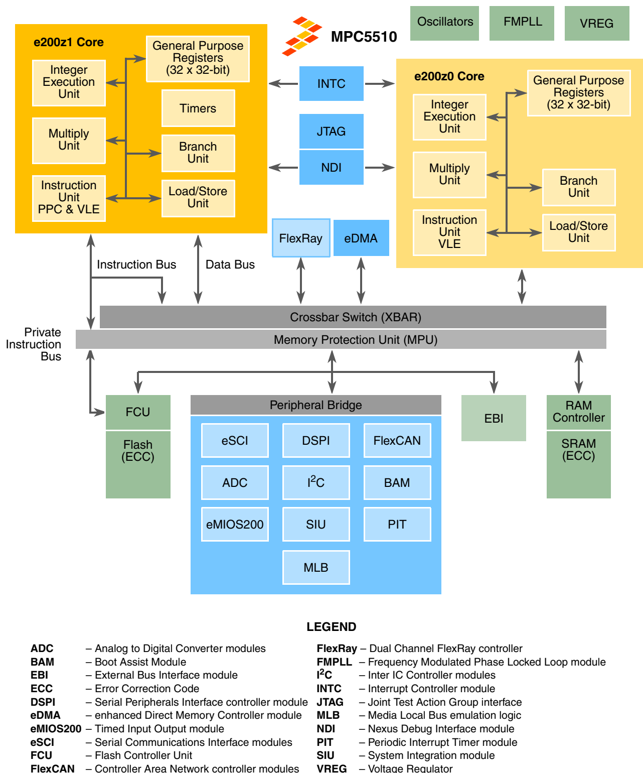
Figure 1. MPC5510 Family Block Diagram
