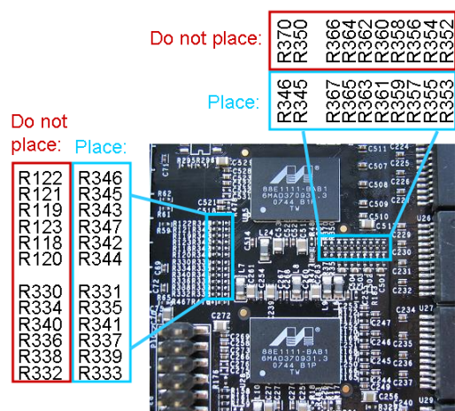
Figure 37. Setup 2 Resistor Options for REVC
