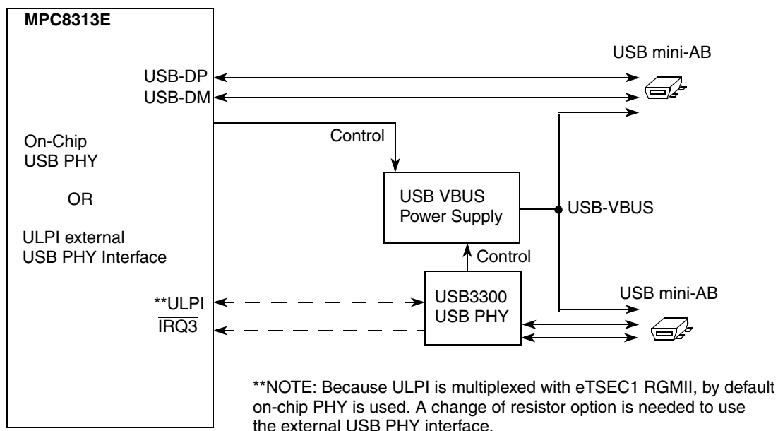
Figure 13. USB Connections
