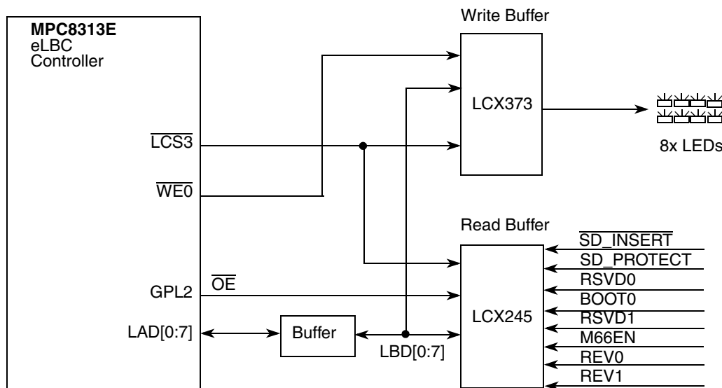
Figure 10. LED/Status Buffers
