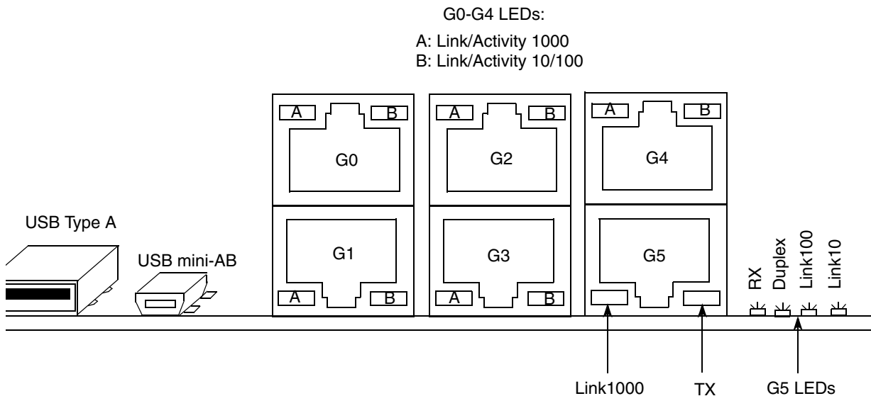
Figure 23. Ethernet Connectors
