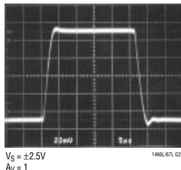
Small-Signal Response V_S = \pm 2.5V
