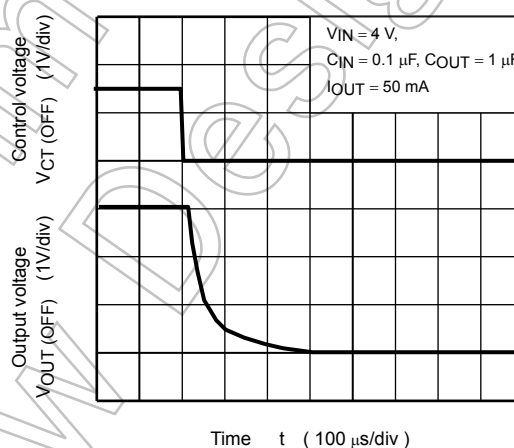
TCR5SB30 (Turn off wave form)
