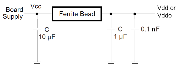
Figure 21. Power-Supply Decoupling
