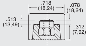
GBFTX turret-type solder pin
