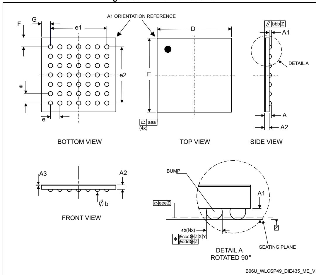
Figure 56. WLCSP49 - Outline
