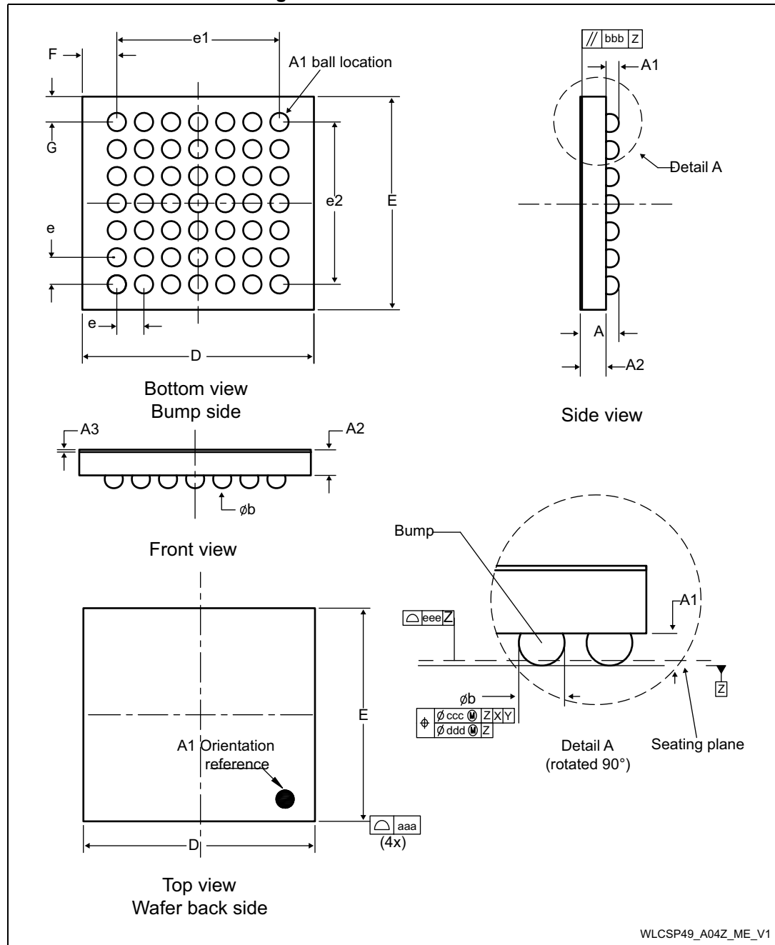
Figure 53. WLCSP49 - Outline
