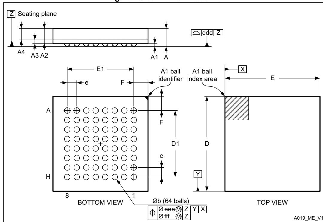
Figure 48. UFBGA64 – Outline
