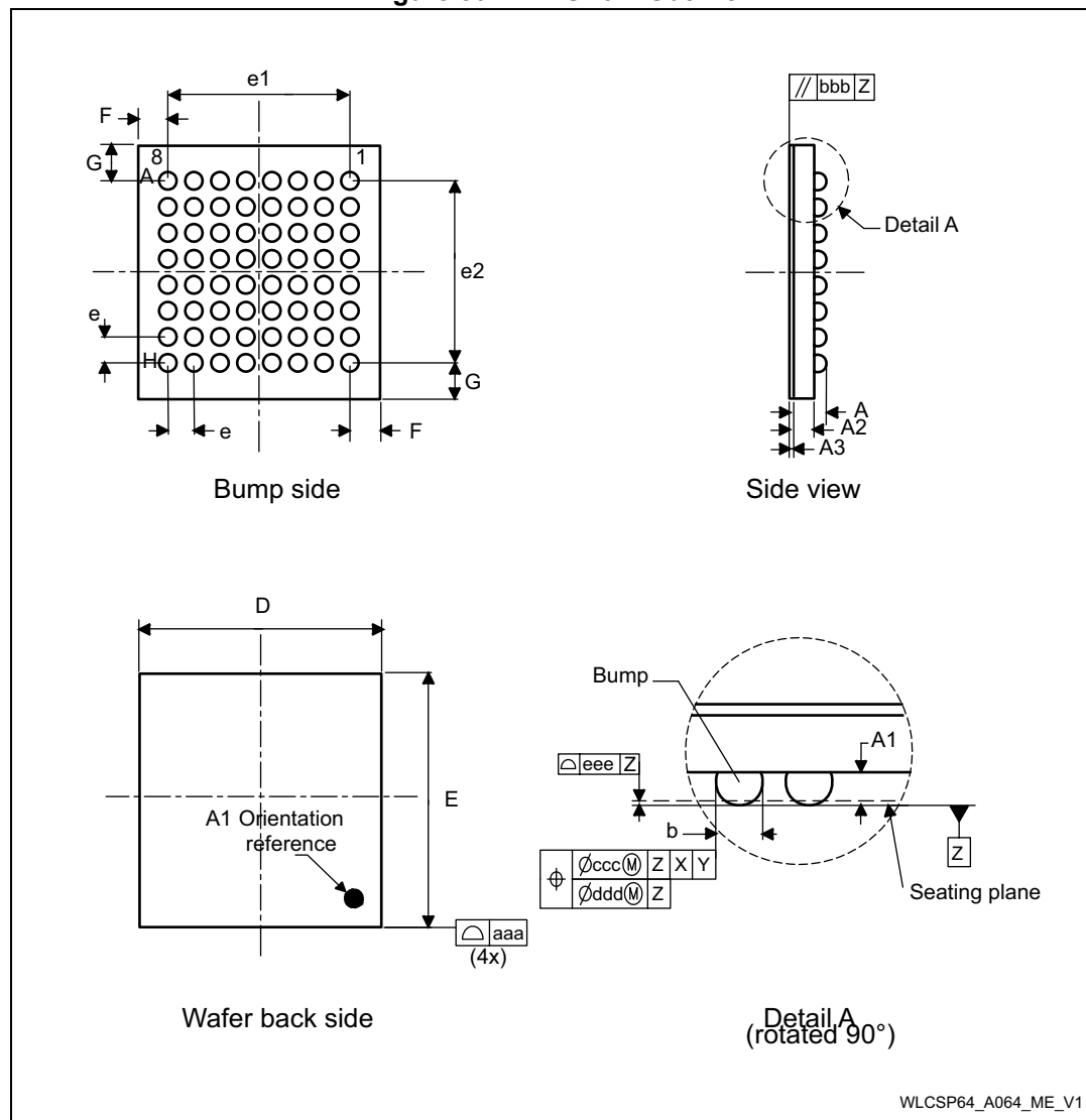
Figure 50. WLCSP64 -Outline
