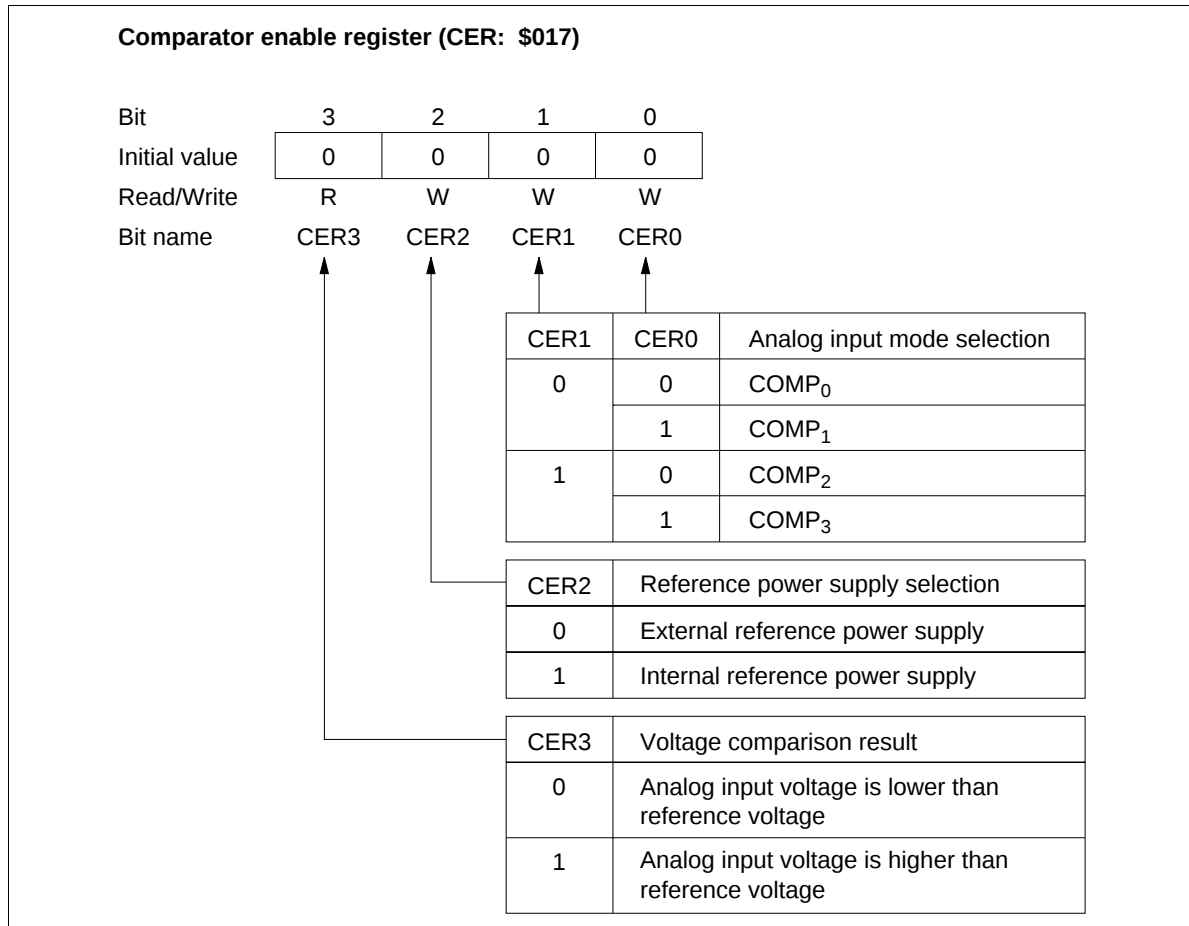
Figure 81 Comparator Enable Register (CER)
