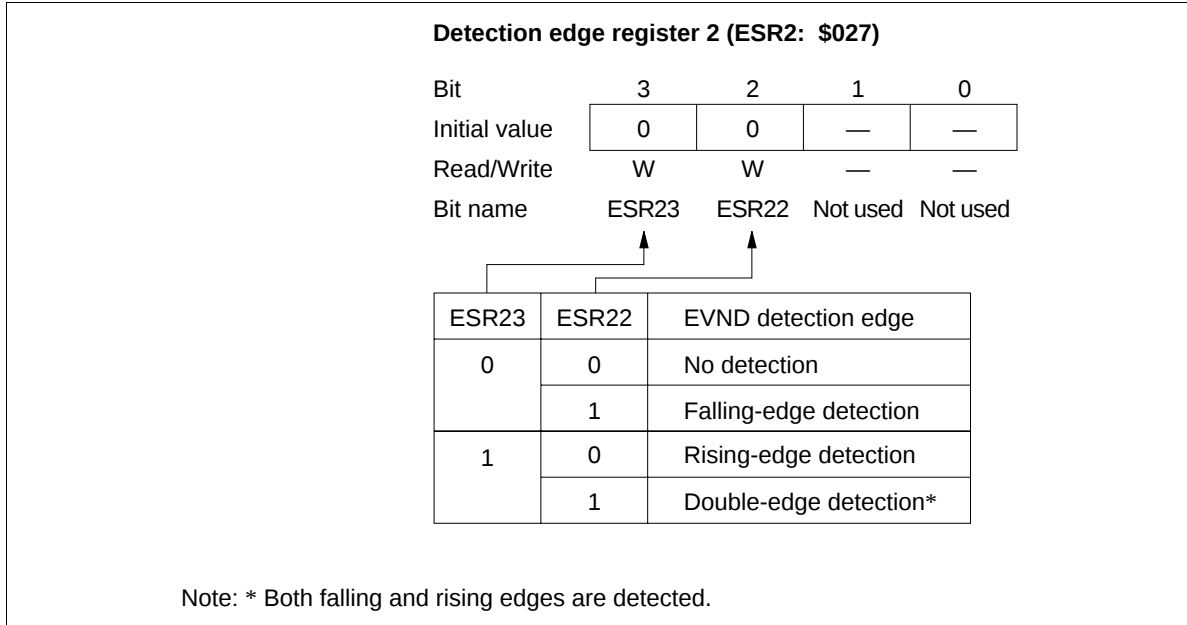
Figure 66 Detection Edge Select Register 2 (ESR2)
