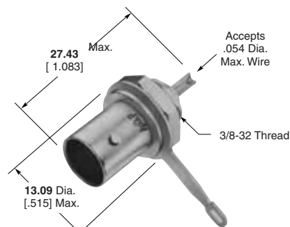
Part No. 5221244-1 (with Solder Terminal)
