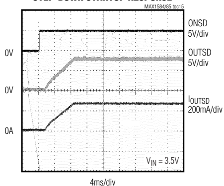
STEP-DOWN STARTUP RESPONSE
