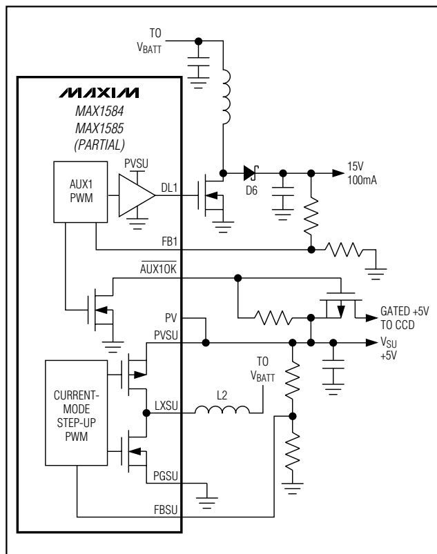
Figure 14. \overline{\text{AUX10K}} drives an external PFET that switches 5V to the CCD only after the +15V CCD bias supply is in regulation.
