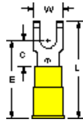
MVU10-10FFBK Stud Size 10 Wire Range 12-10
