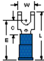
MVU14-8FFBK Stud Size 8 Wire Range 16-14
