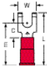
MVU18-8FFBK Stud Size 8 Wire Range 22-18
