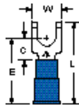
MVU14-10FFBK Stud Size 10 Wire Range 16-14
