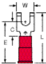
MVU18-6FFBK Stud Size 6 Wire Range 22-18
