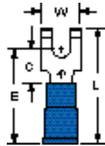
MVU14-6FFBK Stud Size 6 Wire Range 16-14
