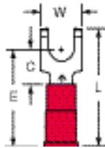
MVU18-10FFBK Stud Size 10 Wire Range 22-18
