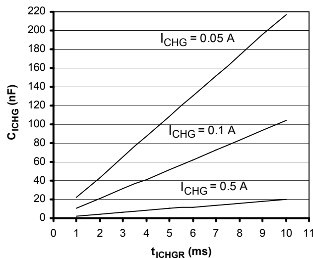
Figure 22. Charging Current External Capacitor ( C_{CHG} ) Versus Charging Current Rise Time ( t_{ICHGR} )
