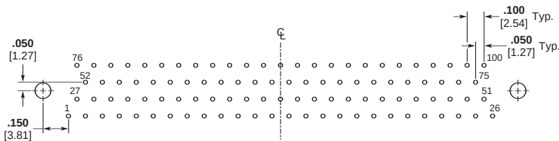
100 Contacts
