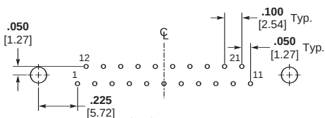
21 Contacts
