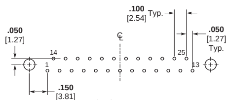
25 Contacts
