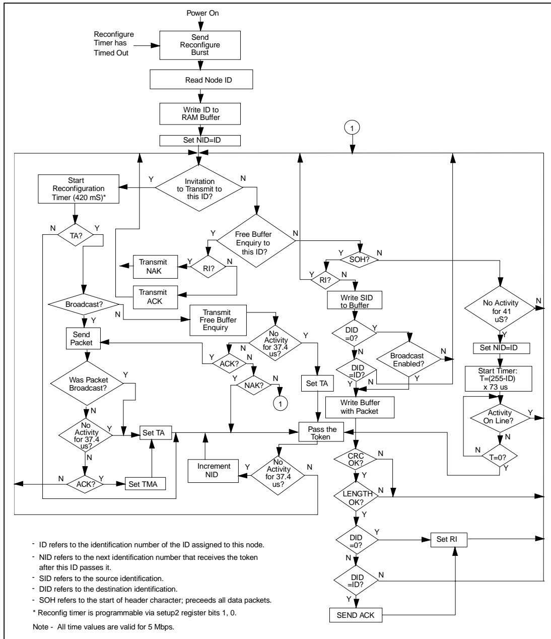
FIGURE 1 - COM20020ID OPERATION
