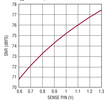
LTC2160: SNR vs SENSE, f_{IN} = 5\text{MHz} , -1\text{dBFS}
