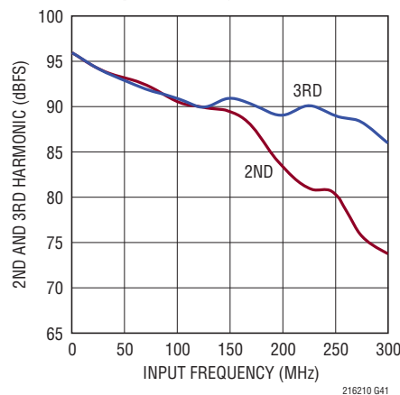
LTC2160: 2nd, 3rd Harmonic vs Input Frequency, -1\text{dBFS} , 25\text{Mps} , 1\text{V} Range
