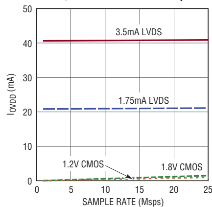
LTC2160: I_{OVDD} vs Sample Rate, 5\text{MHz} , -1\text{dBFS} Sine Wave Input
