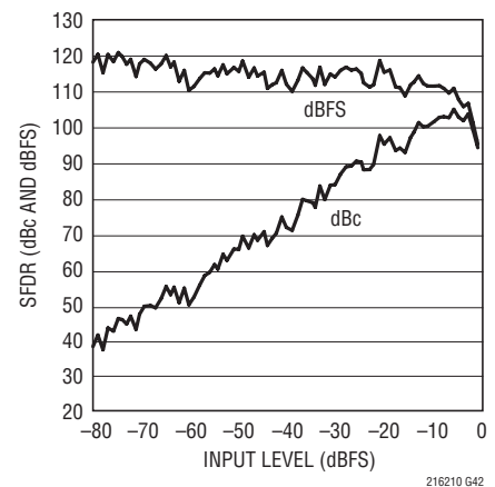
LTC2160: SFDR vs Input Level, f_{IN} = 70\text{MHz} , 25\text{Mps} , 2\text{V} Range
