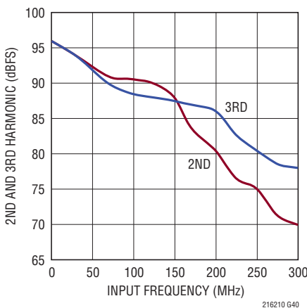
LTC2160: 2nd, 3rd Harmonic vs Input Frequency, -1\text{dBFS} , 25\text{Mps} , 2\text{V} Range
