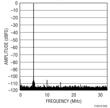
LTC2162: 64k Point FFT, f_{IN} = 5\text{MHz} , -1\text{dBFS} , 65Msps
