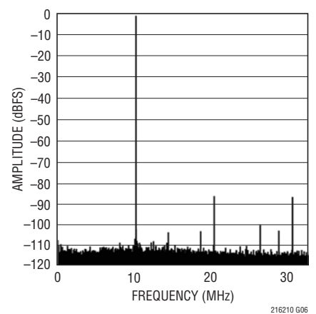
LTC2162: 64k Point FFT, f_{IN} = 140\text{MHz} , -1\text{dBFS} , 65Msps
