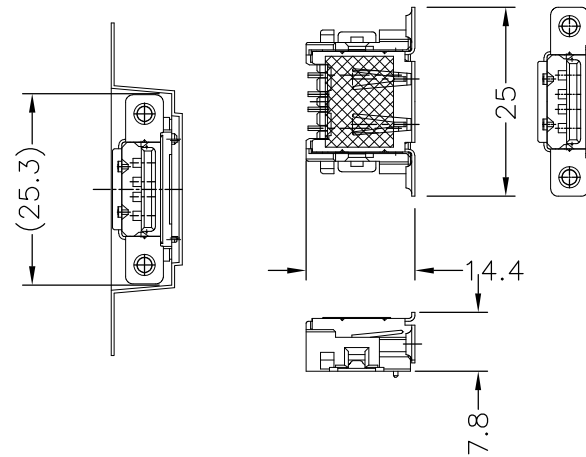
CONNECTOR DETAIL
