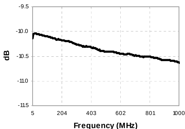
Coupling: pin 6 - pin 4
