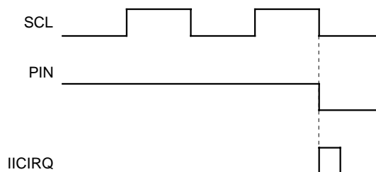
Fig. 8.6.8 Interrupt Request Signal Generation Timing
